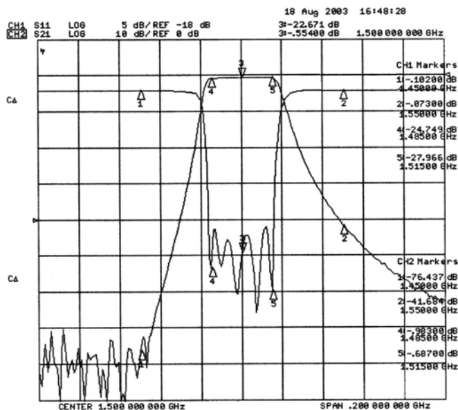
Passband Response
